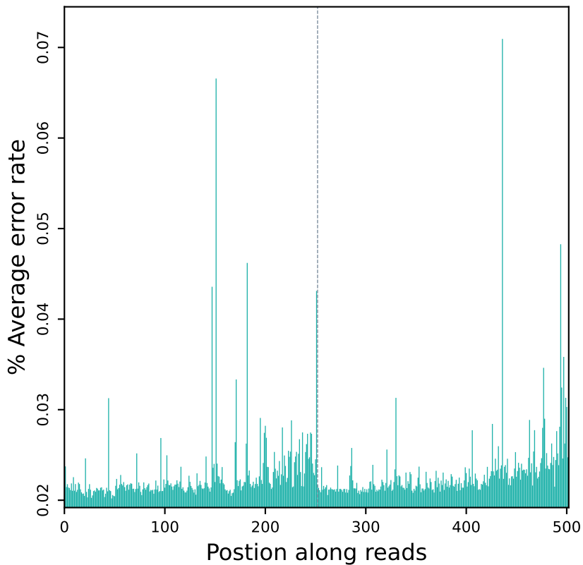
Error rate distribution along reads (R10606)
